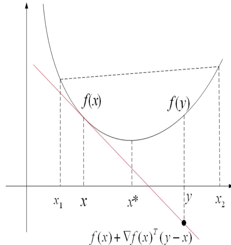
Convex function
